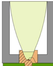
Spotlight LED design
